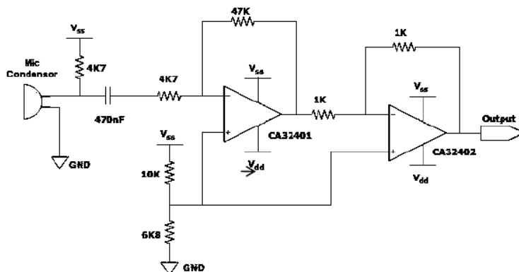
Gambar 2. Rangkaian Pre-Amplifier (Sumber : Huda et al.,2019)
