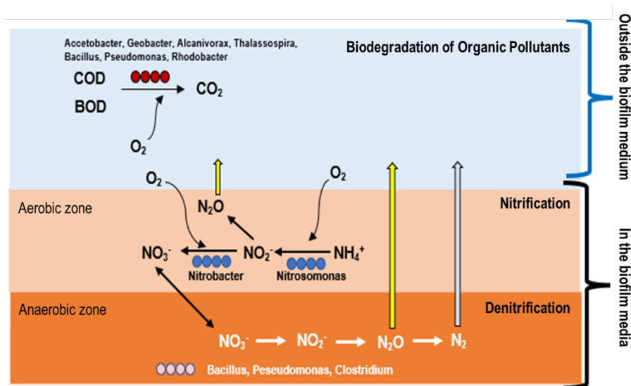
Figure 2. MBBR reaction process (Source: Muharja et al., 2022)
